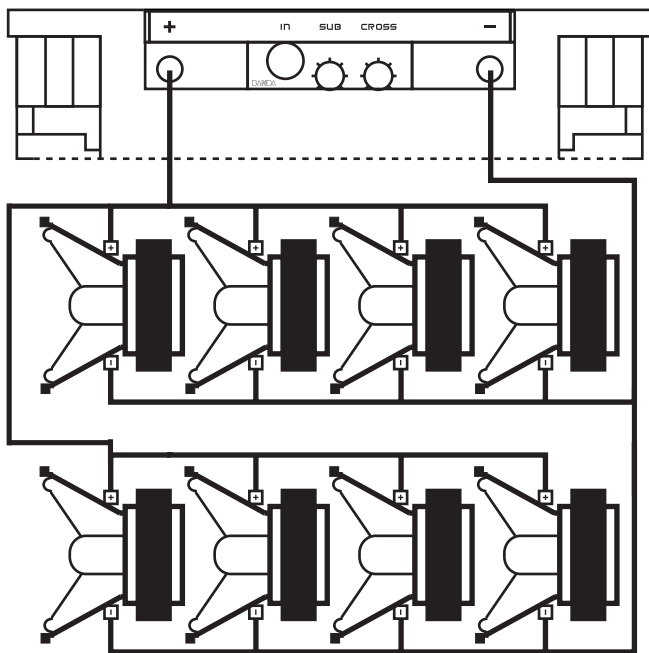
8 ohms 1250Wrms woofer x 8 wired in parallel
