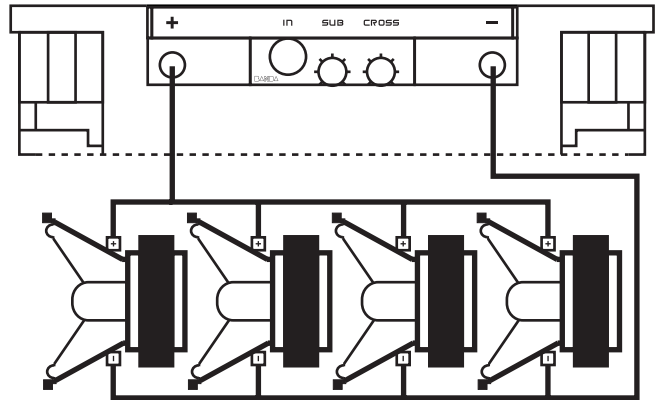
4ohms 2500Wrms woofer x 4 wired in parallel
