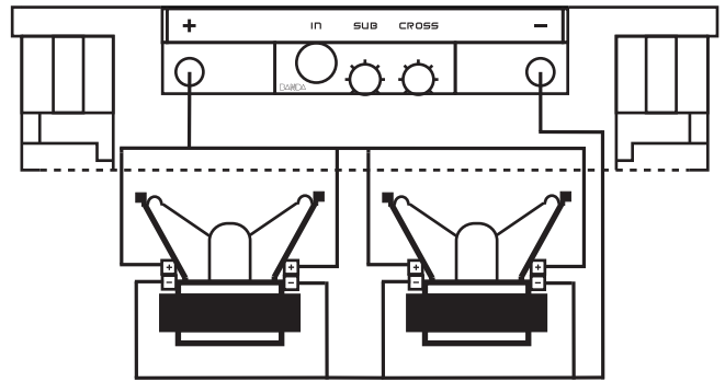
4+4ohms 5000Wrms subwoofer x 2 wired in parallel
